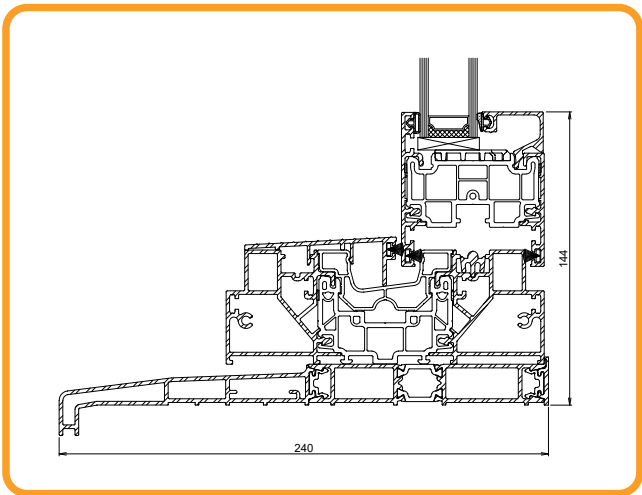
STANDARD OUTER FRAME WITH 240MM CILL
